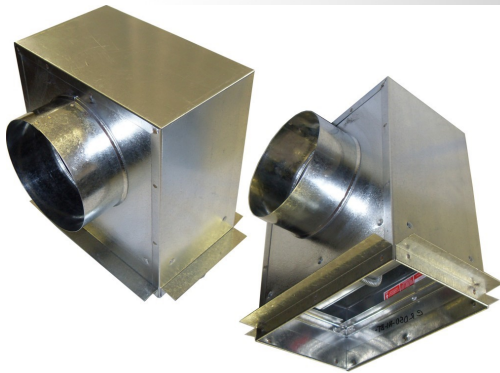
TYPE CRD: Rectangular damper with non-insulated galvanized steel register box
