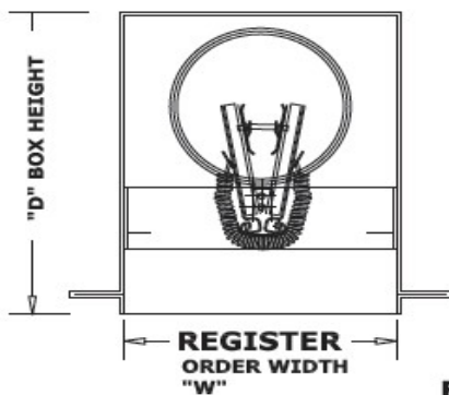
TYPE CRD: Rectangular damper with non-insulated galvanized steel register box
