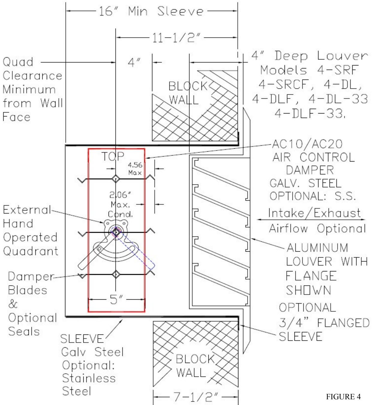
FIGURE 4 ILLUSTRATES THE COMBINATION OF LOUVER/ AIR CONTROL DAMPER/ SLEEVE/ QUADRANT FOR 4" DEEP 4-SRF & 4-SRCF, 4-DL, 4-DLF LOUVERS FOR INSTALLATION INTO 7-1/2" BLOCK WALLS ** (Min. sleeve length depends on the wall thickness)
