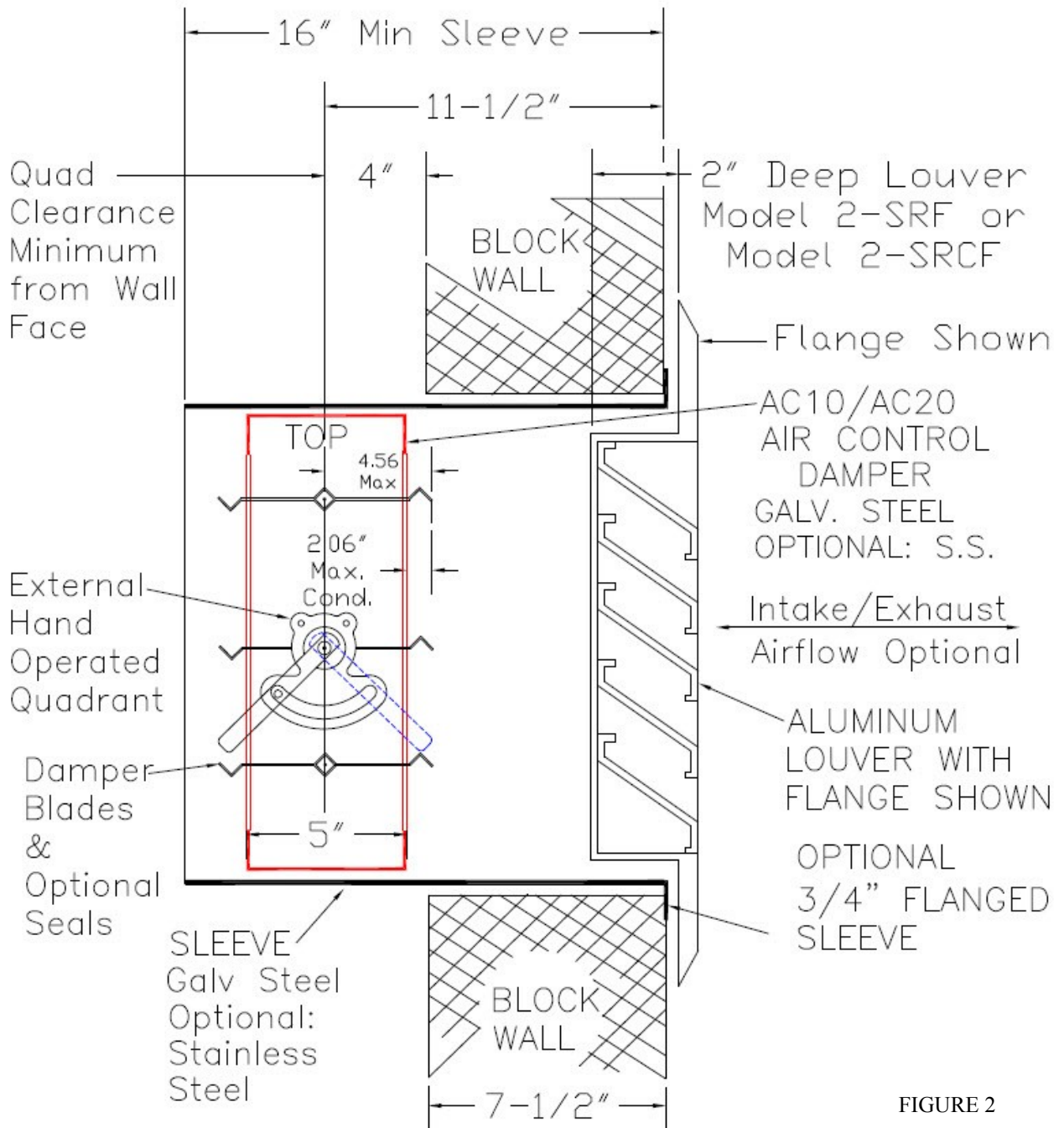
FIGURE 2 ILLUSTRATES THE COMBINATION OF LOUVER/ AIR CONTROL DAMPER/ SLEEVE/ QUADRANT FOR 2" DEEP 2-SRF & 2-SRCF LOUVERS FOR INSTALLATION INTO 7-1/2" BLOCK WALLS **(Min. sleeve length depends on the wall thickness)
